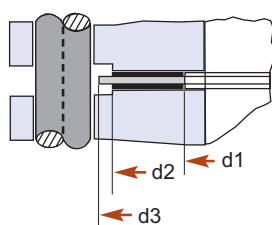
STYLE ZG & ZA To Suit ASME B16.5 and BS 1560 Flanges Class 150 up to 2500
